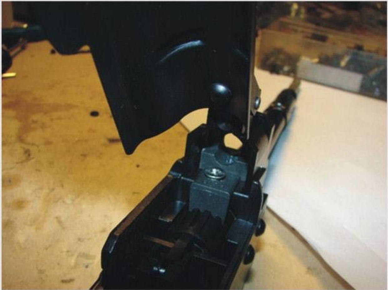
STEP15: The finish of hop-up unit and inner barrel.
